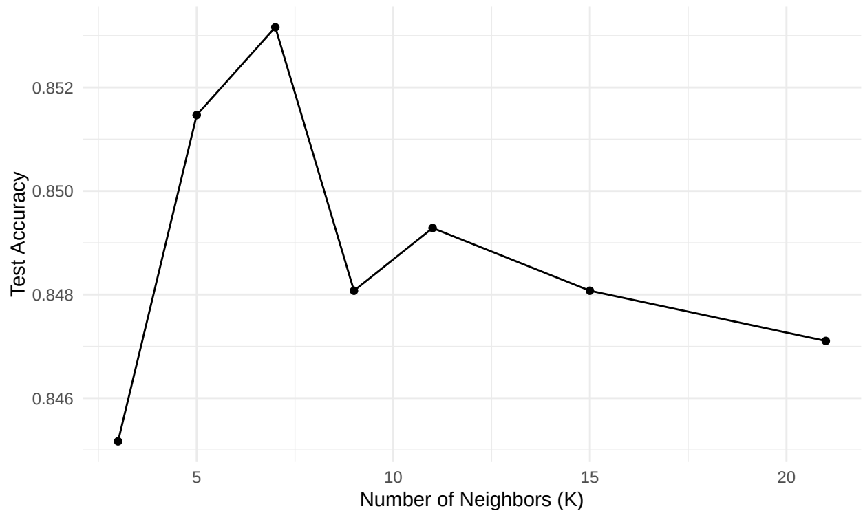
KNN Accuracy Across Different K Values
